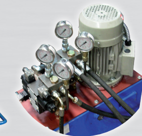
UNIT WITH ELECTROVALVES
